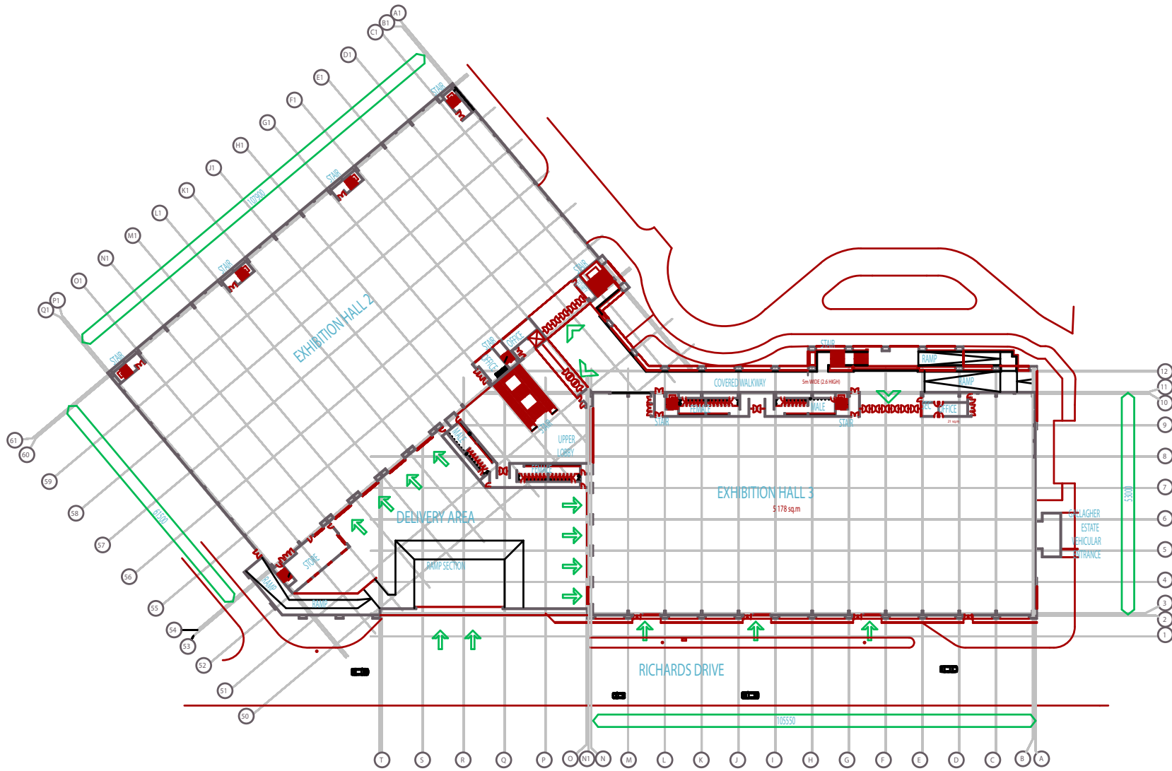
UPPER LEVELS - OVER ALL FLOOR PLAN
